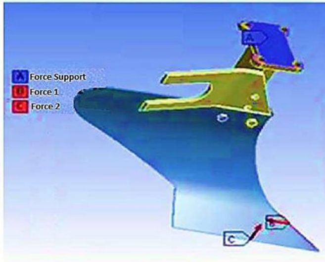
Fig. 6. Determining the place of application of force and support in the reversible plow
