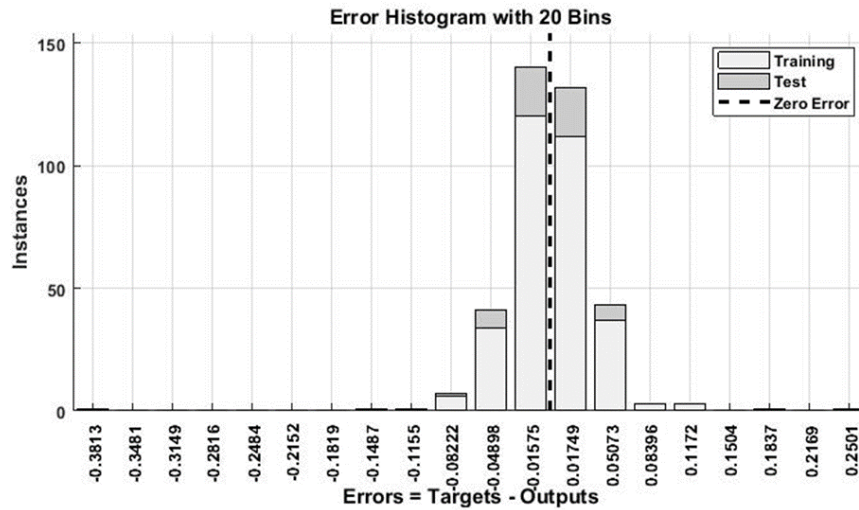
Fig. 12. Histogram of Von Meikes stress prediction error by neural network
