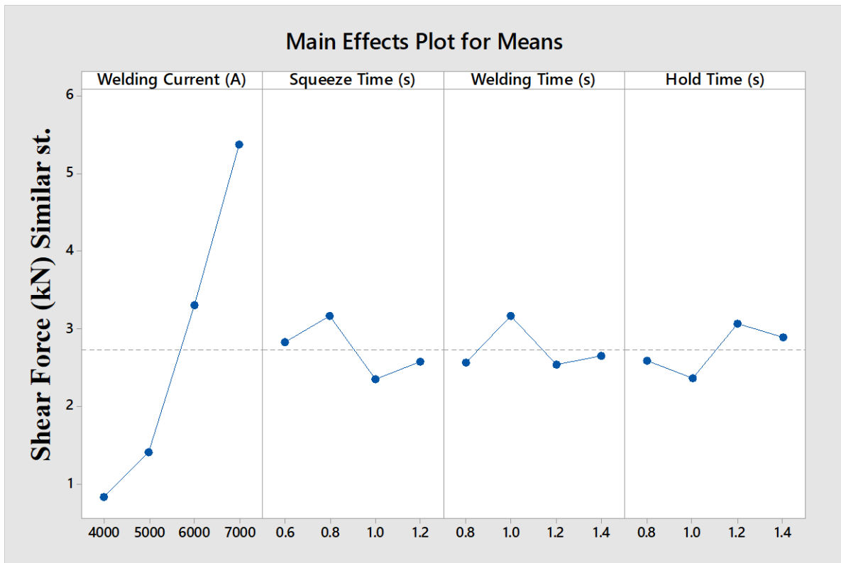
Fig. 8. Main effect plot of AISI 1005
