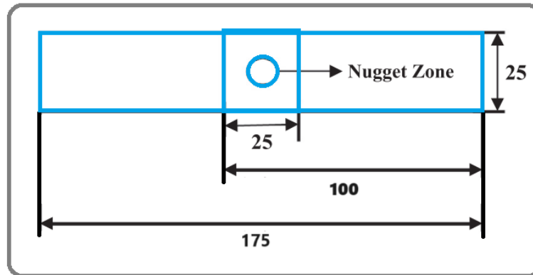
Fig. 2. Test specimen dimension (in mm)
