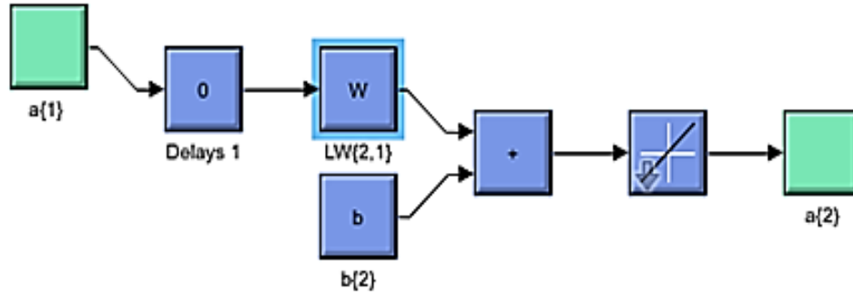
Fig. 12. Second layer processing
