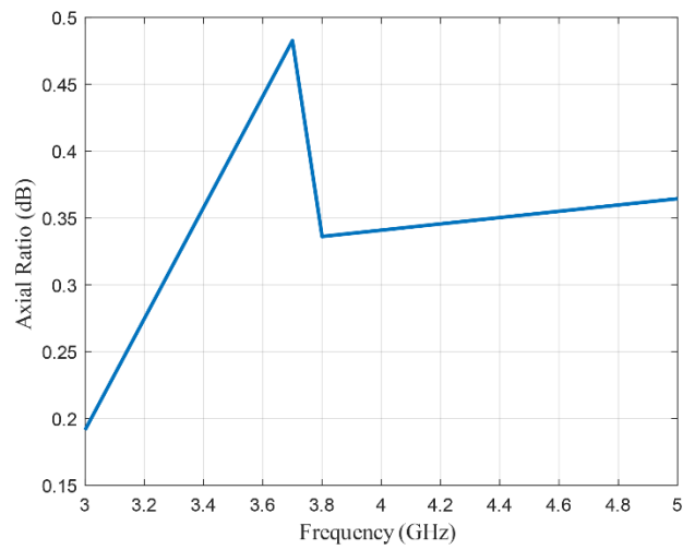
Fig. 5 AR for single antenna element
