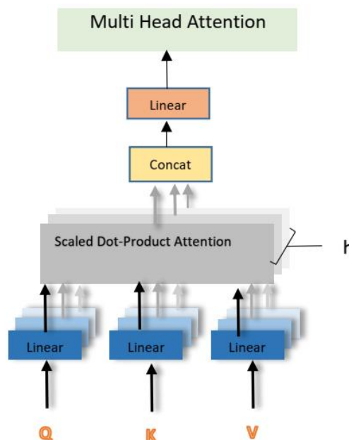
Fig. 4. Multi-Head Attention architecture
